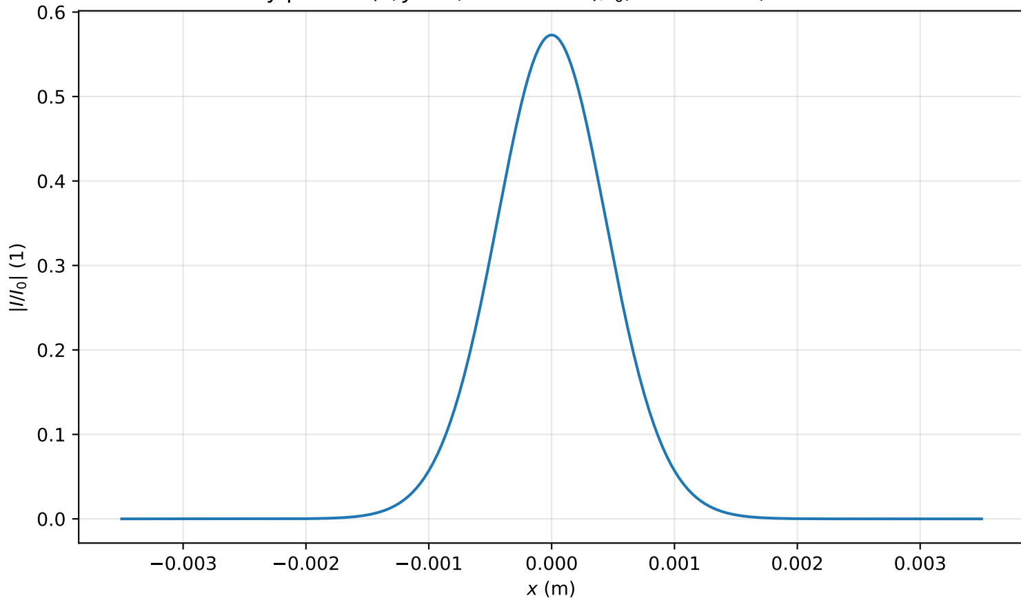
Intensity profile I(x, y = 0, z = 2.070m)/I_0 , P_{in}=0.2P_{cr} , artificial time
